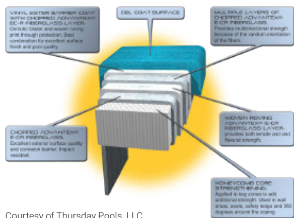
Figure 1 Laminate schedule – fiberglass swimming pool fabrication
