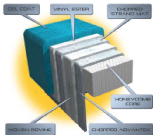
Figure 2 Laminate schedule – fiberglass swimming pool fabrication
